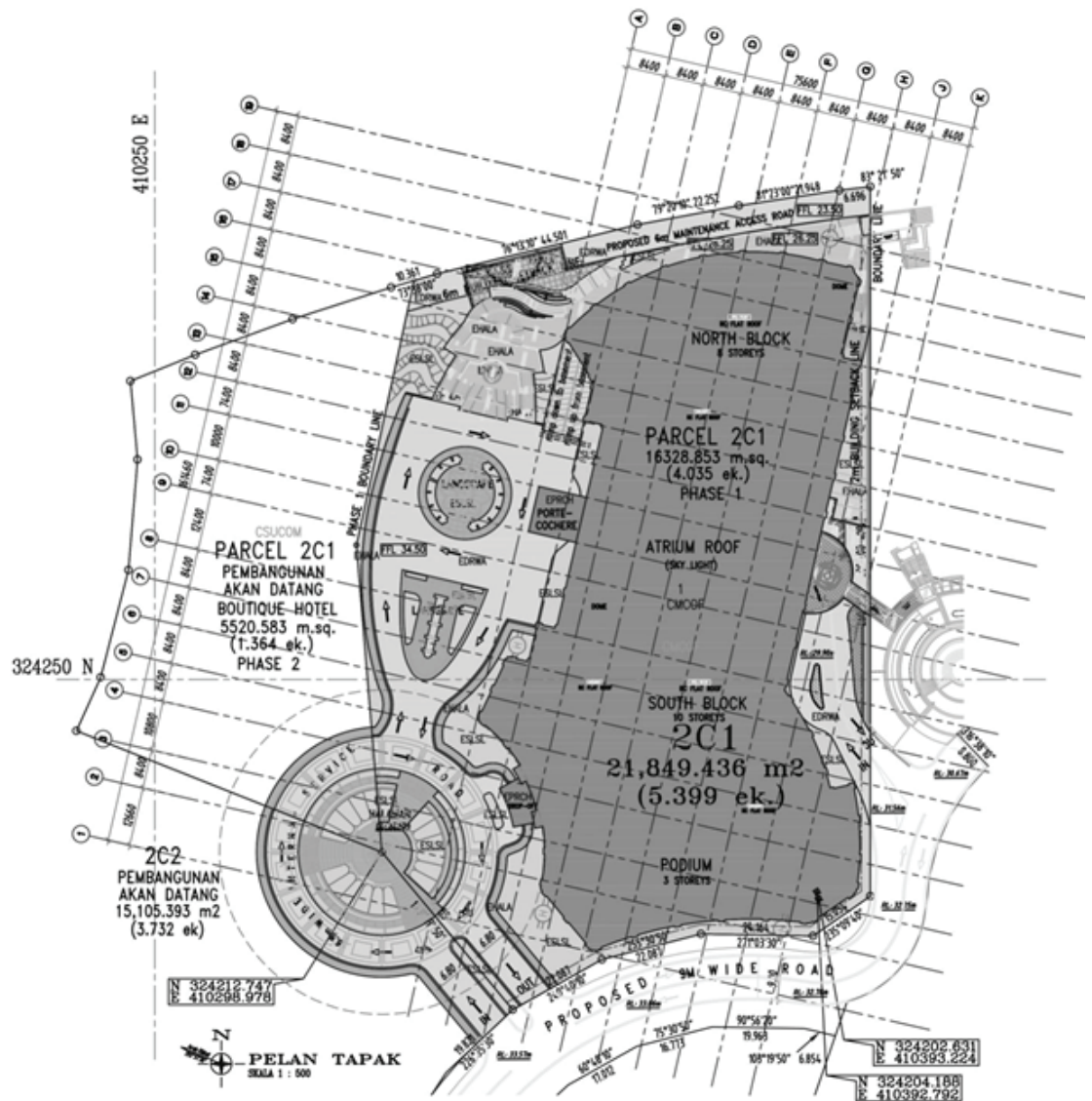
Figure 4: Site plan of Menara Seri Wilayah (Source: Jabatan Perancangan Bandar, Perbadanan Putrajaya) Interview with the architect on his idea of a national architectural identity for the building
