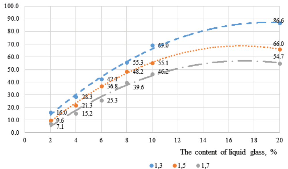
Figure 1: The dependence of the strength characteristics of slag cement from the content of liquid glass silicate with different modules.
