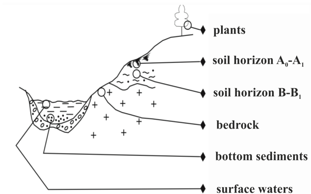
Figure 1: A system of conjugated components of the geological environment.
