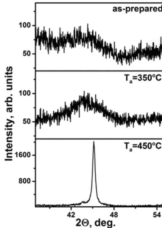
Figure 3: XRD patterns of the film of Fe_{72.5}Si_{14.2}B_{8.7}Nb_2Mo_{1.5}Cu_{1.1} alloy in as-prepared state and at different annealing temperatures.
