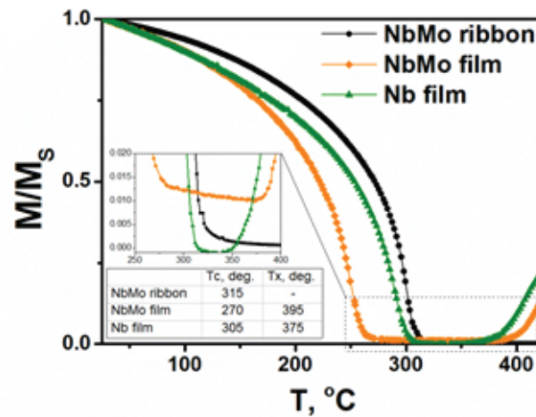
Figure 2: Temperature dependences of M for of Fe_{73.9}Si_{13.2}B_{8.9}Nb_3Cu_1 alloy film and of Fe_{72.5}Si_{14.2}B_{8.7}Nb_2Mo_{1.5}Cu_{1.1} alloy film and ribbon.
