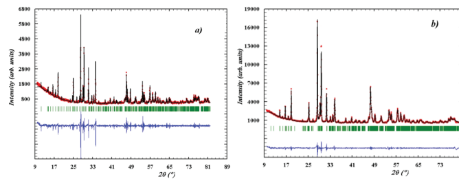
Figure 1: XRD patterns Gd_2(WO_4)_3 , Ho_2(WO_4)_3 .
