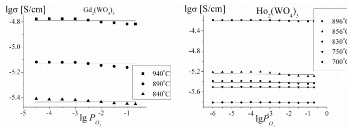
Figure 4: Oxygen pressure dependence of conductivity for \text{Ln}_2(\text{WO}_4)_3 .
