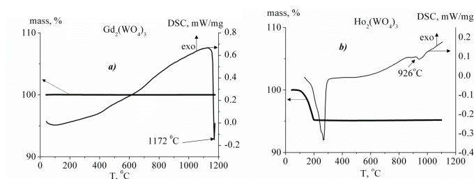
Figure 2: TGA and DSC results for Ln_2(WO_4)_3 .
