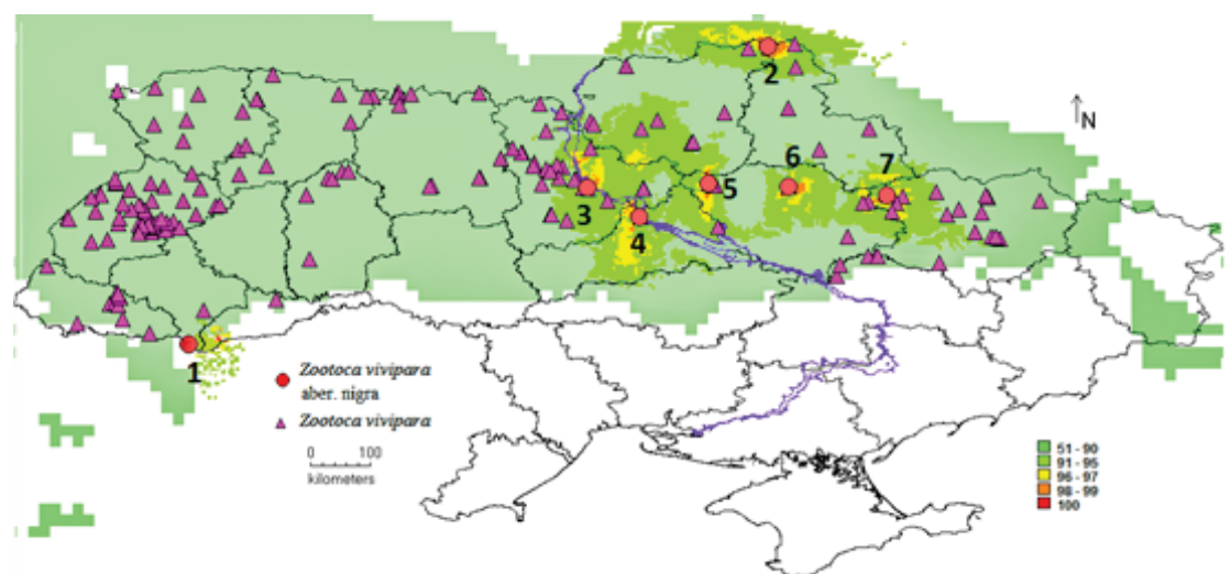
Figure 1: The results of GIS modeling of potential distribution of Z. vivipara (DIVA-GIS and Maxent) (No. 1-7 marking in the text).
