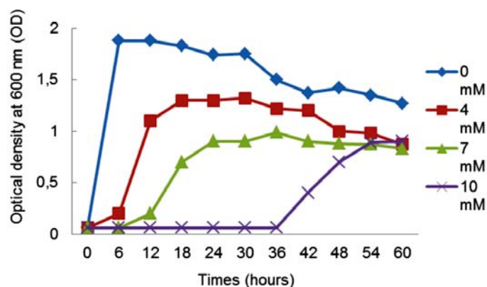
Figure 1. The growth of Cupriavidus sp. IrC4 in medium containing various concentration of \text{CuSO}_4
