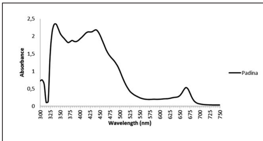
Figure 4. Spectrum absorbance of Phaeophyta extracted using acetone 90%
