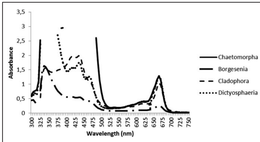
Figure 1. Spectrum absorbance of Chlorophyta extracted using acetone 90%
