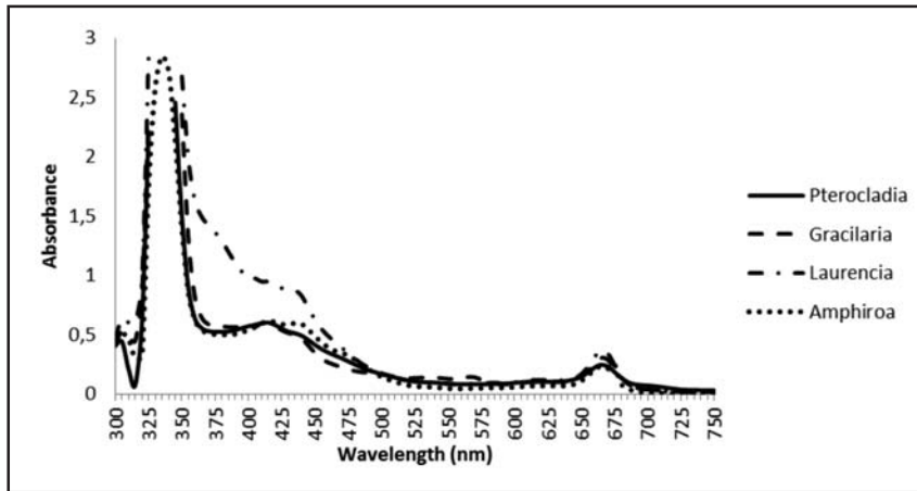
Figure 3. Spectrum absorbance of Rhodophyta extracte using acetone 90%
