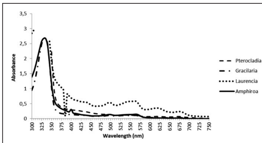
Figure 2. Spectrum absorbance of Rhodophyta extracted using aquadest
