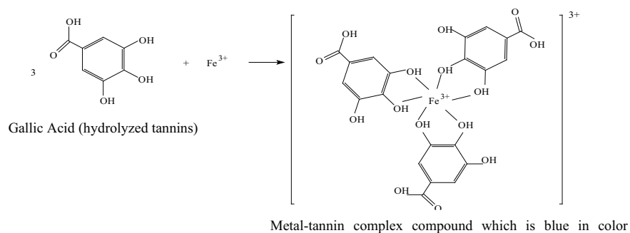
Figure 4: Complex compound formation reaction between Tannin and FeCl 3 proposed [19].
