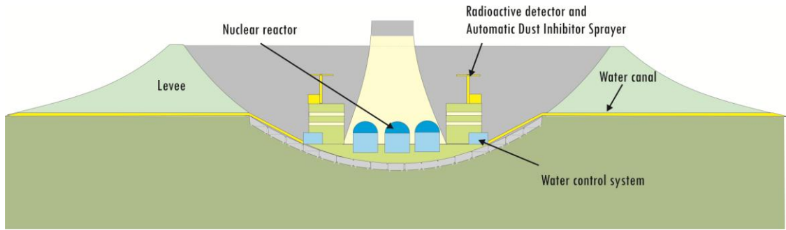
Fig. 1. The concept of nuclear power plant with Ball in Bowl design.
