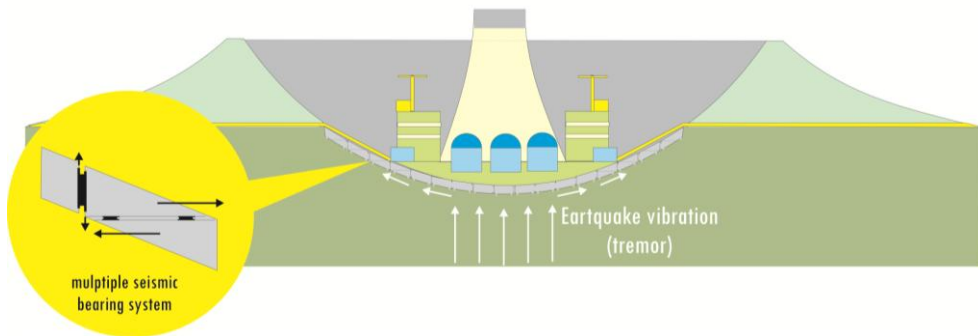
Fig. 4. Earthquake protection mechanism.
