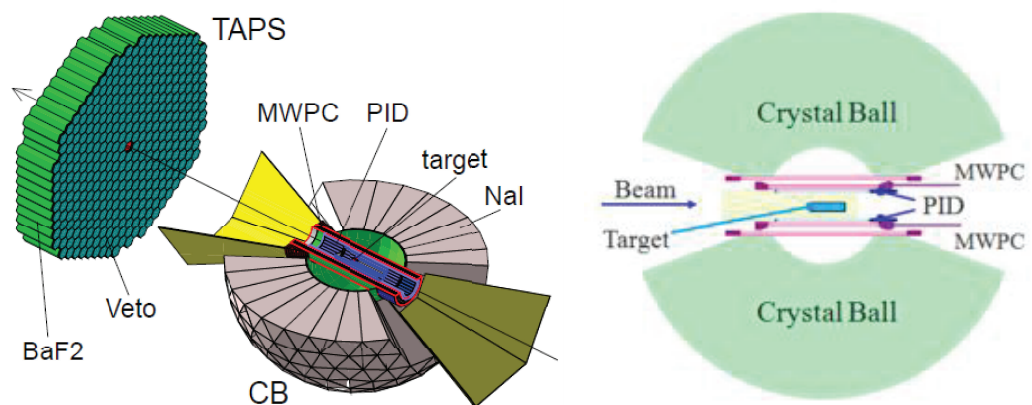
Figure 1: Left: layout of the A2 detector systems. Right: expanded view of the target region.
